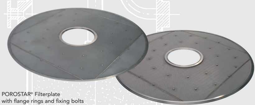
POROSTAR® Filterdiscs Dimensions: \varnothing 2.4 mm up to 3 m Applications: Chromatography, Plastic melt filtration
